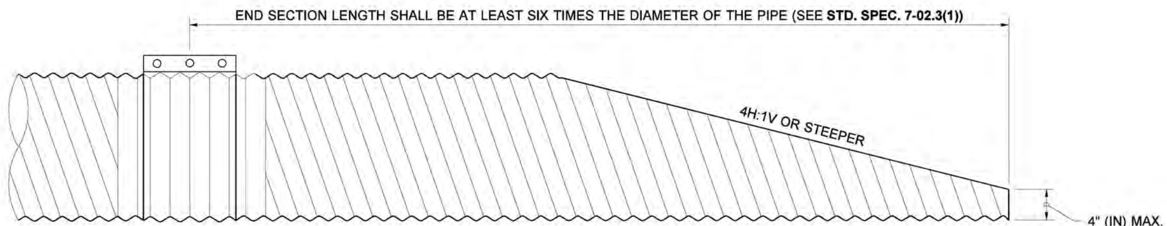
METAL PIPE
