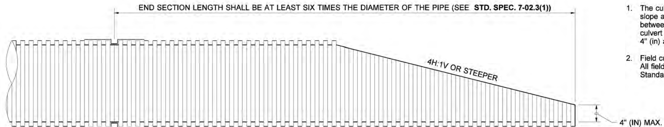
THERMOPLASTIC PIPE
