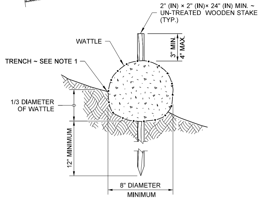
WATTLE DETAIL
