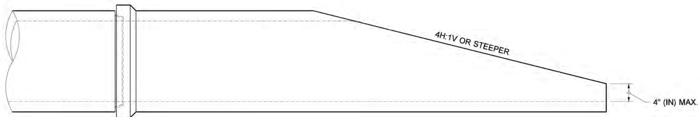
CONCRETE PIPE
