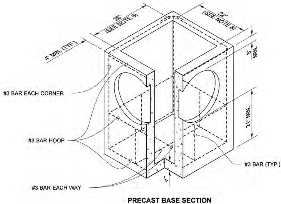
PRECAST BASE SECTION
